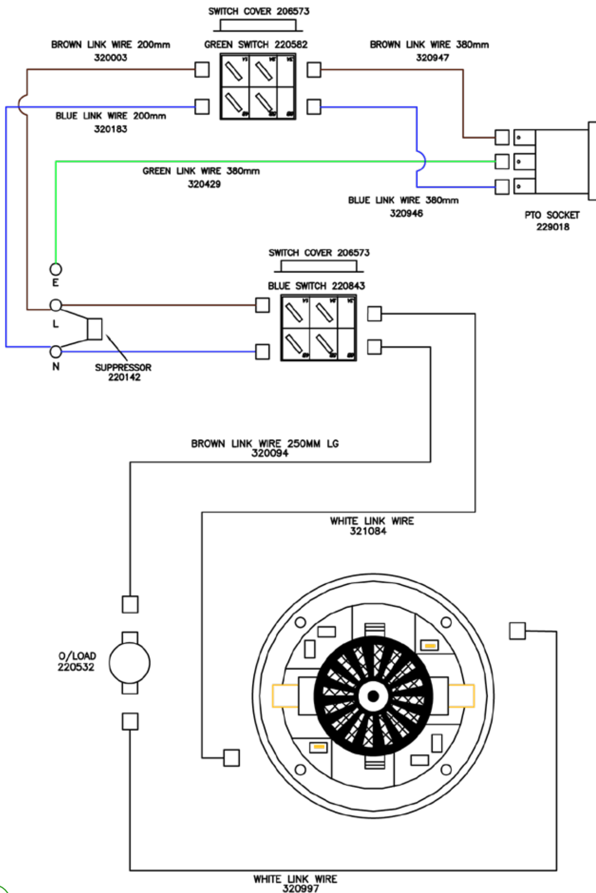
Wiring Diagram
