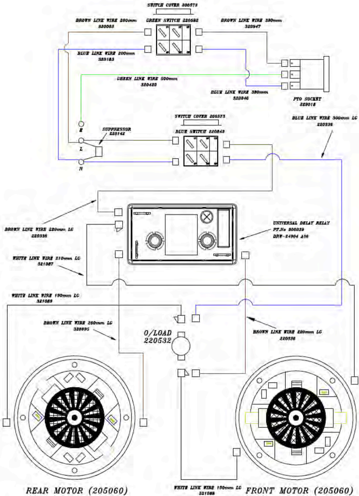
Wiring Diagram
