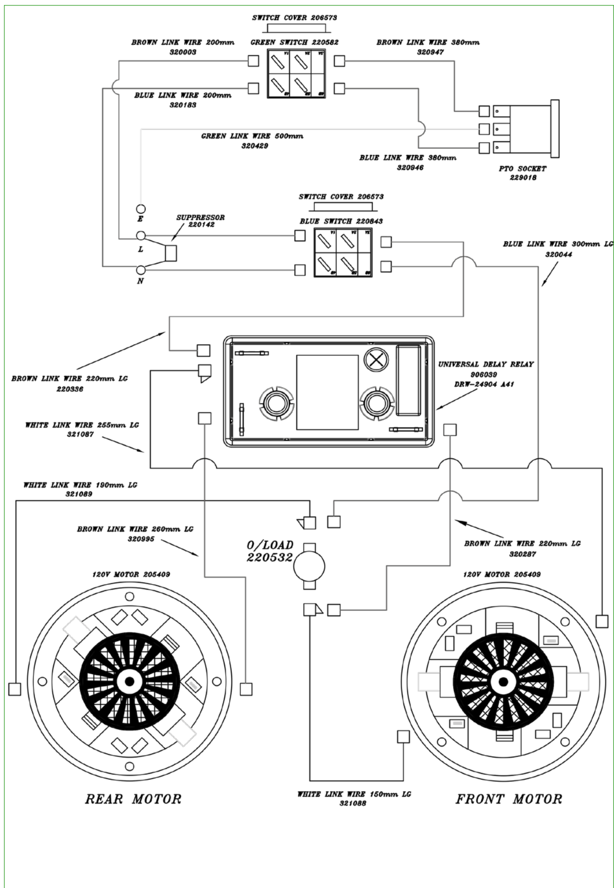
Wiring Diagram
